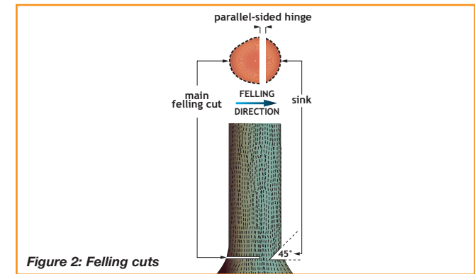
Figure 2: Felling cuts
